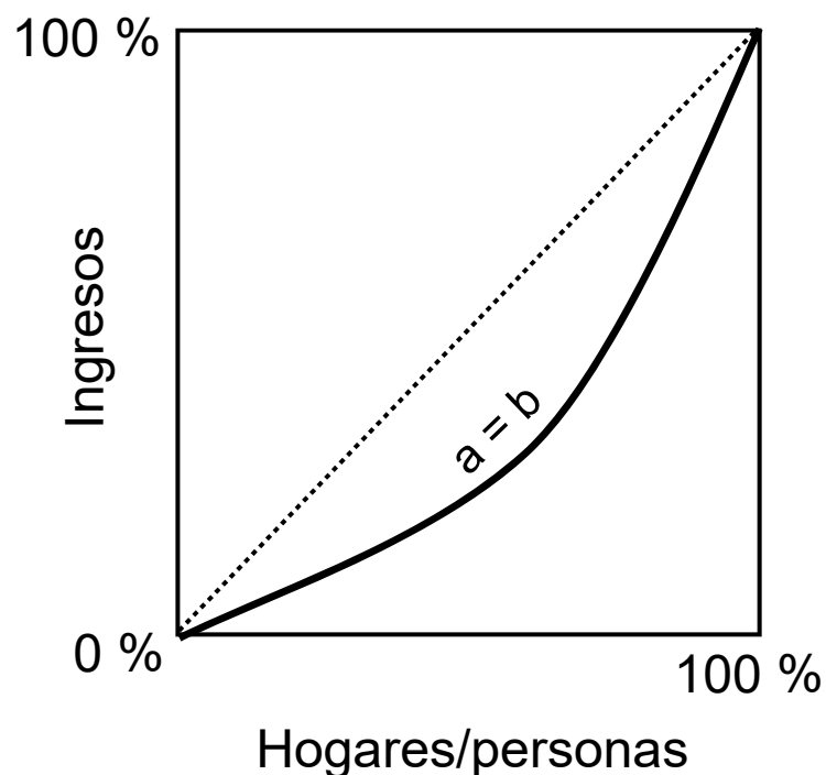
Curva de Lorenz a = b
